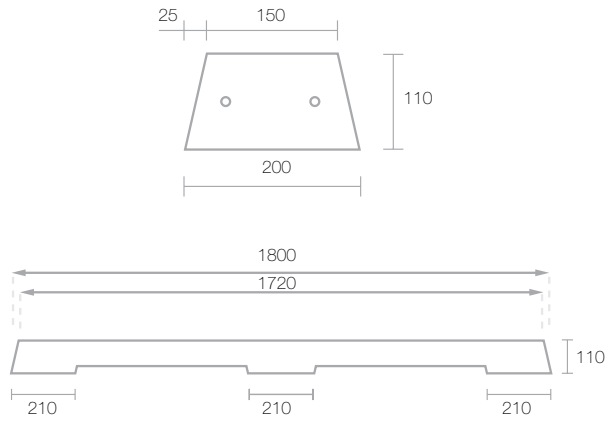
JAGAS low profile car buffer
