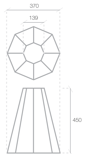
JAGAS octagonal bollard
