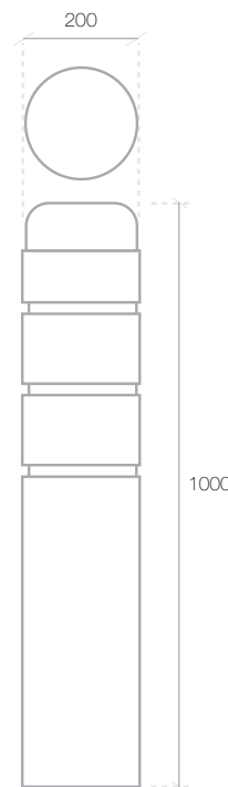
JAGAS round bollard Type 40
